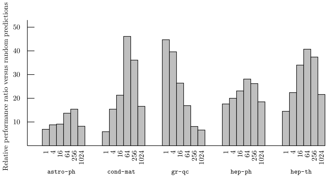
Figure 10: Relative performance of the low-rank matrix-entry predictor for various ranks on each arXiv section. For each arXiv section, the performance of this predictor, measured by the factor of improvement over random predictions, is shown for ranks 1, 4, 16, 64, 256, and 1024. Notice that for all arXiv sections save gr-qc , predictor performance is maximized by an intermediate rank; for that data set, performance continues to improve as the rank decreases all the way to rank one.
